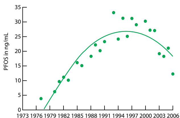
Figure 3.33. Temporal trends in concentrations of PCBs (sum of five congeners, ng/g fat; top graph), PBDEs (sum of seven congeners, ng/g fat; middle graph), and PFOS (ng/mL; bottom graph) in pooled ( n > 20 ) serum samples from Norwegian men. PCB, PBDE and PFOS concentrations were measured in the same group of men (Thomsen, Liane & Becher, 2007; Haug, Thomsen & Becher, 2009).
