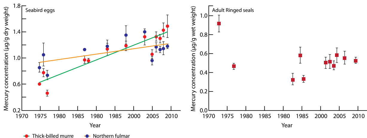
Figure 3.26. Temporal trends in concentrations of mercury in seabird eggs ( \mu\text{g/g dry weight} ; Braune et al. 2010) and ringed seal muscle ( \mu\text{g/g wet weight} ; Gaden et al. 2009; Muir et al. 2011) from the Canadian Arctic archipelago.
