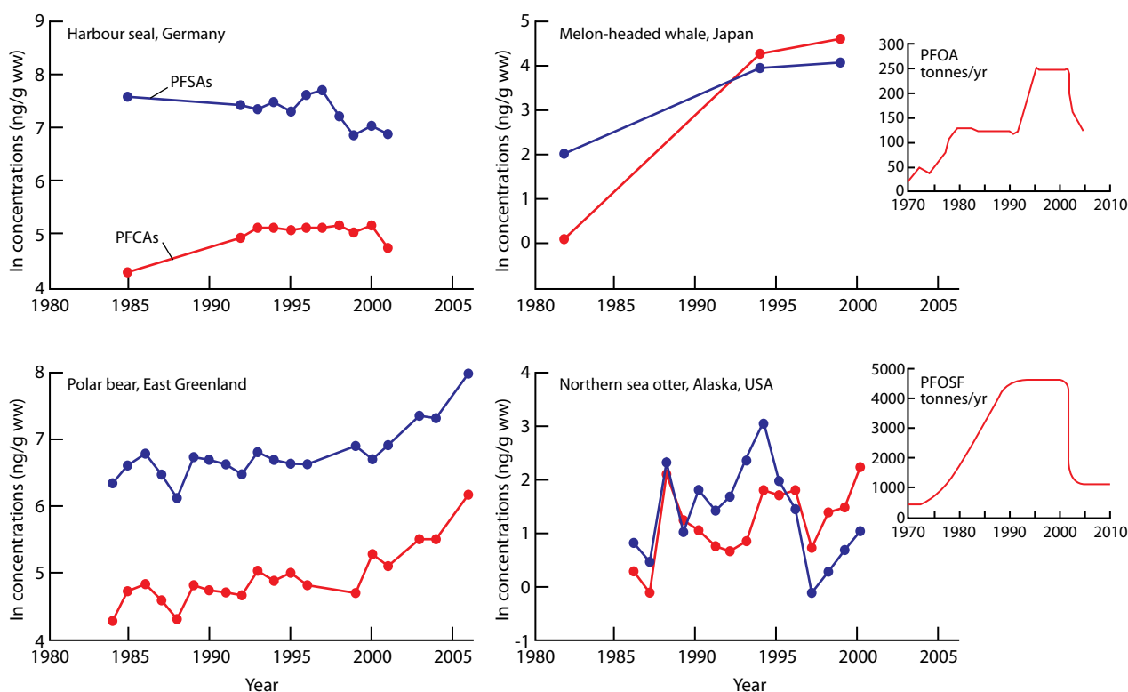
Figure 3.24. Temporal trends in concentrations (ng/g wet weight) of perfluorinated carboxylates (PFCAs) and perfluorinated sulfonates (PFASs) in tissues of marine mammals (Houde et al., 2011). Inserted graphs: Estimated maximum global emissions of PFOA (Armitage et al., 2006) and estimated total global production of PFOSF, the major PFOS starting material (Paul, Jones & Sweetman, 2009). Composite figure based on the references given.
